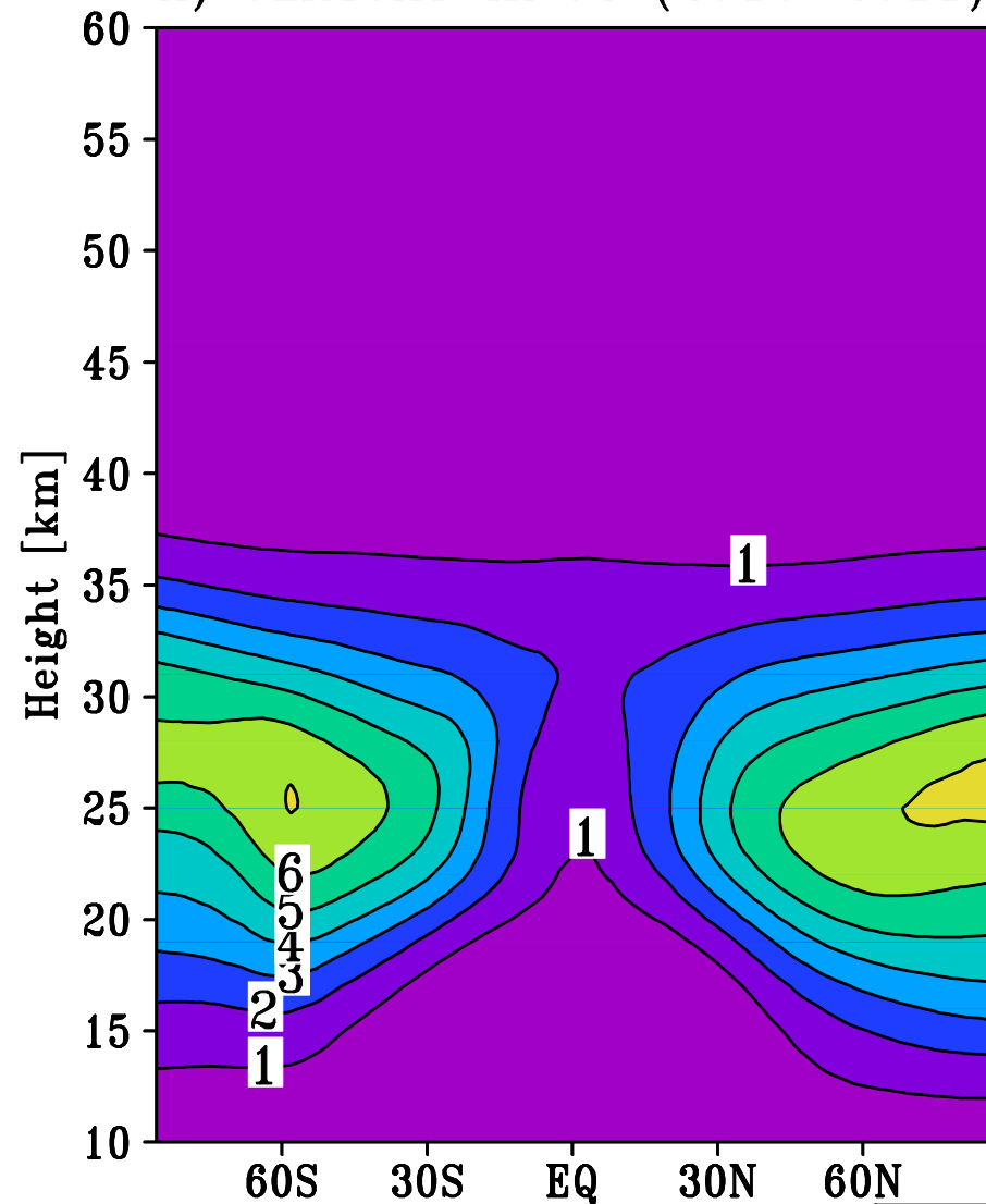
A) SLIMCAT HN03 (2010–2011)
