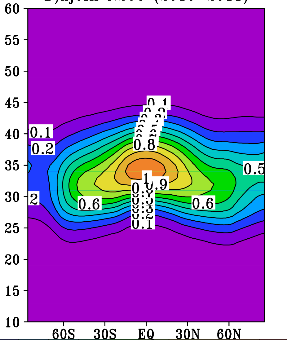
B) xjcin N205 (2010–2011)
