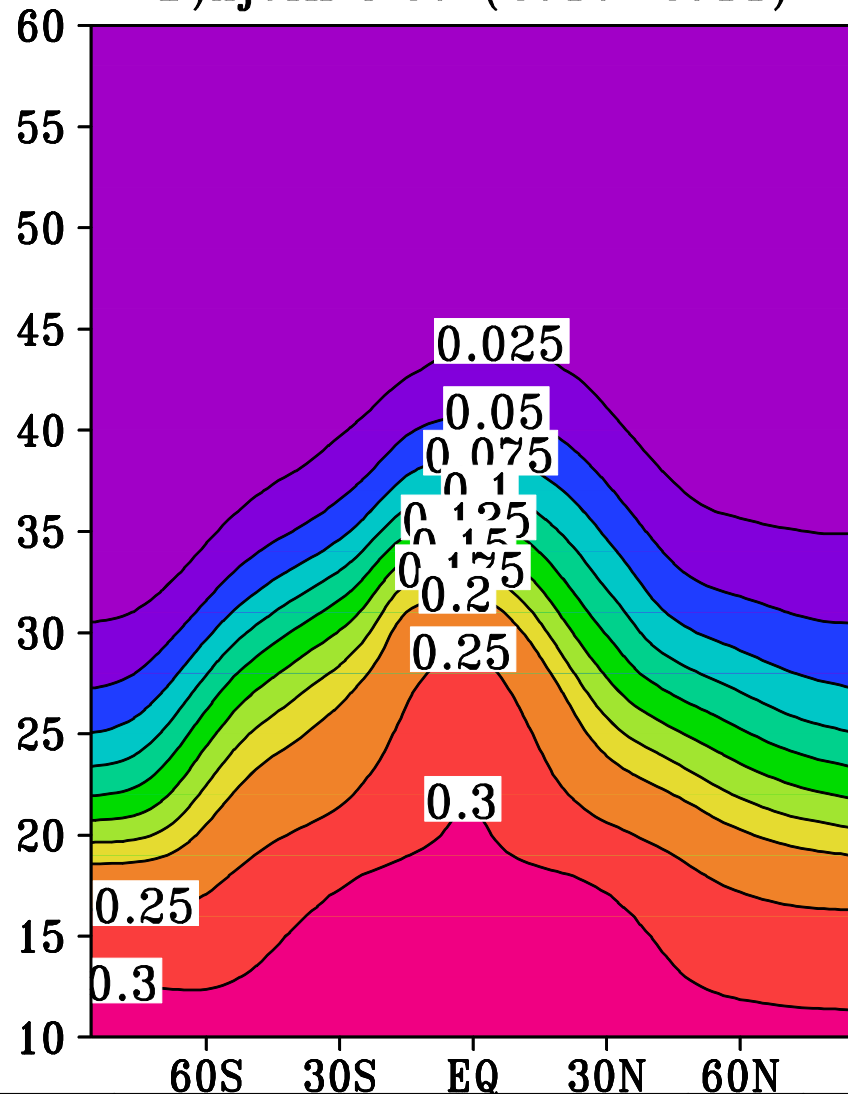
B) xjcin N2O (2010–2011)
