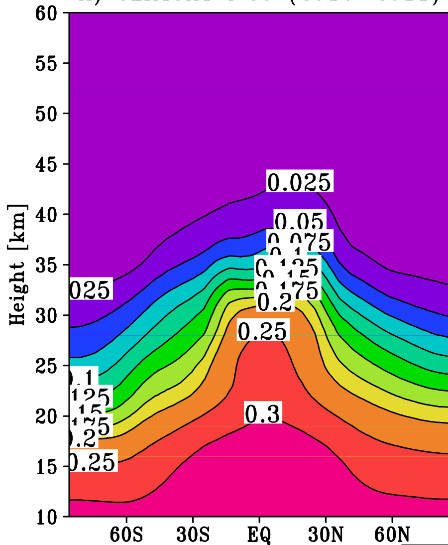
A) SLIMCAT N2O (2010–2011)
