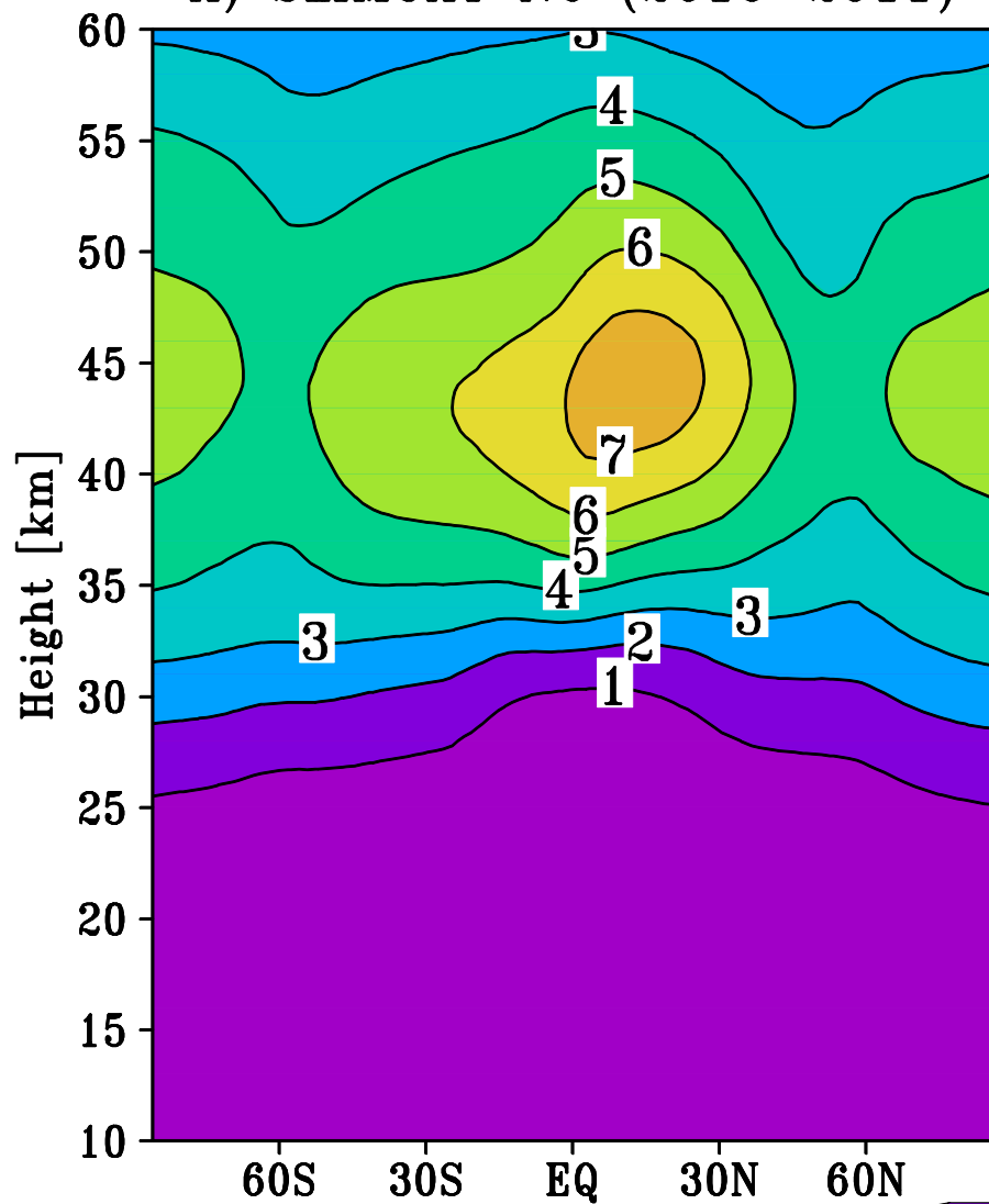
A) SLIMCAT NO (2010–2011)
