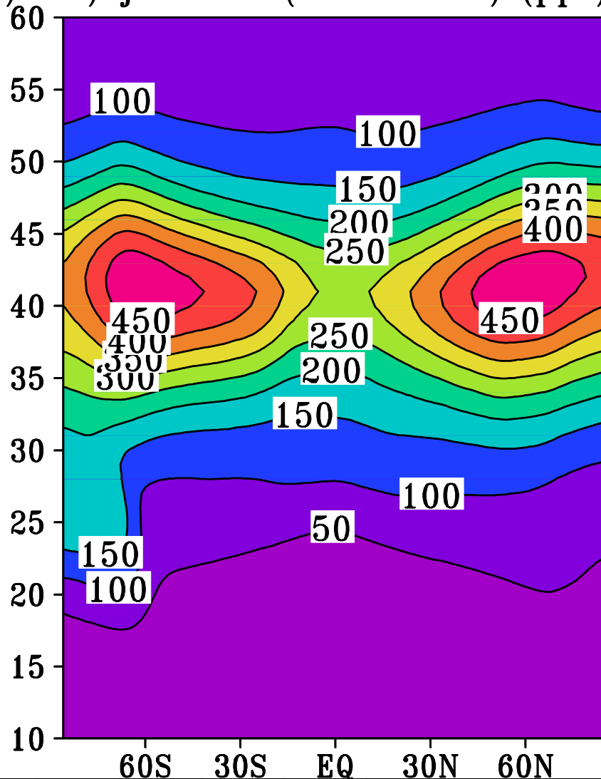
B) xjcin ClO (2010–2011) (ppt)
