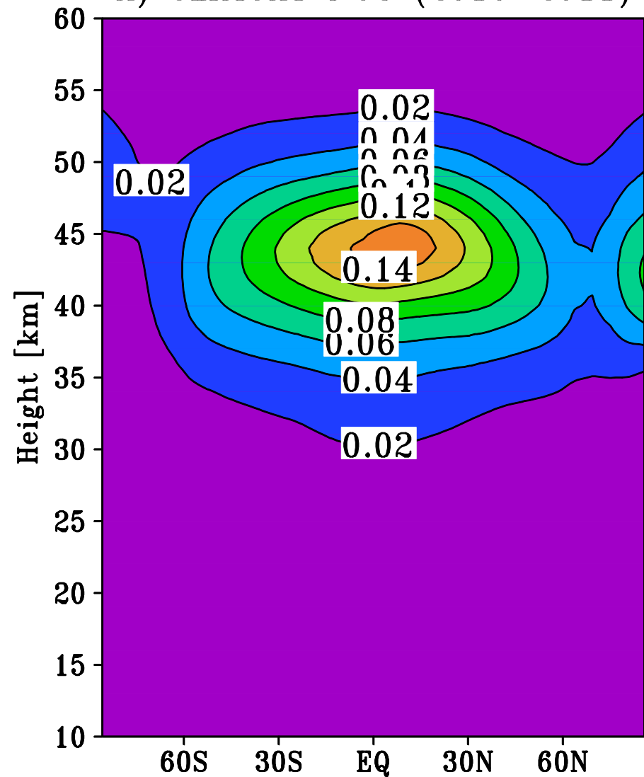
A) SLIMCAT N03 (2010–2011)
