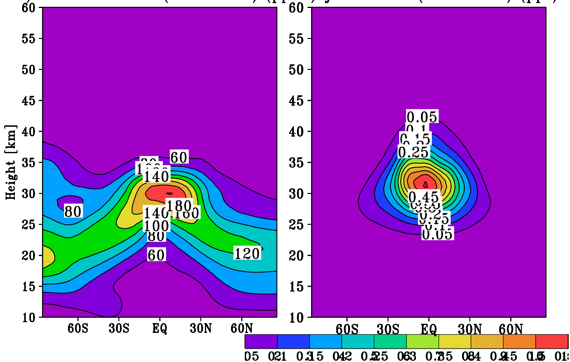
A) SLIMCAT H 2 SO 4 (2010–2011) (ppt) B) xjcin H 2 SO 4 (2010–2011) (ppt)
