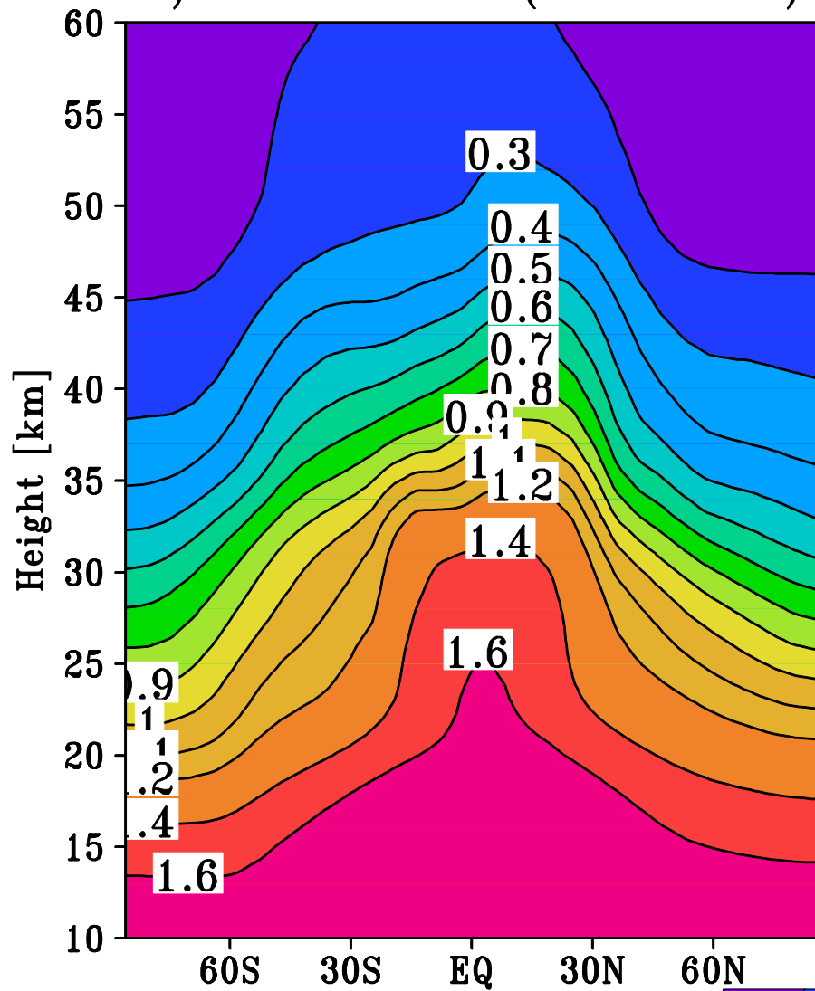
A) SLIMCAT CH 4 (2010–2011)
