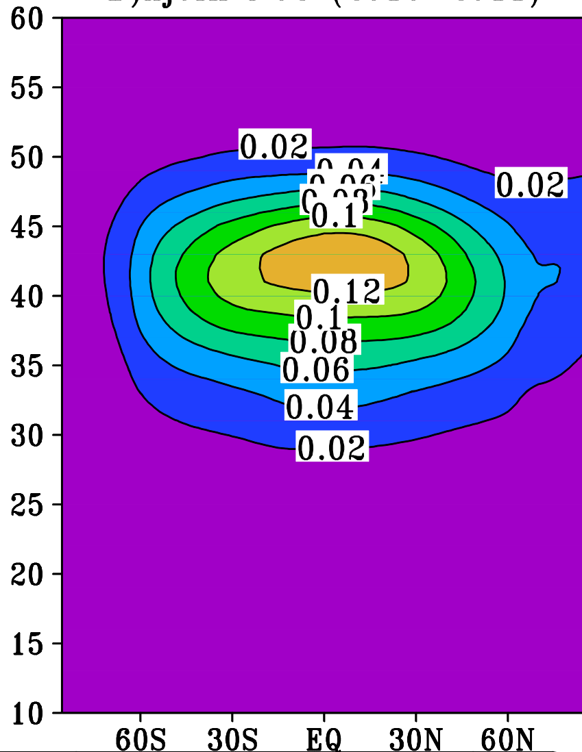
B) xjcin N03 (2010–2011)
