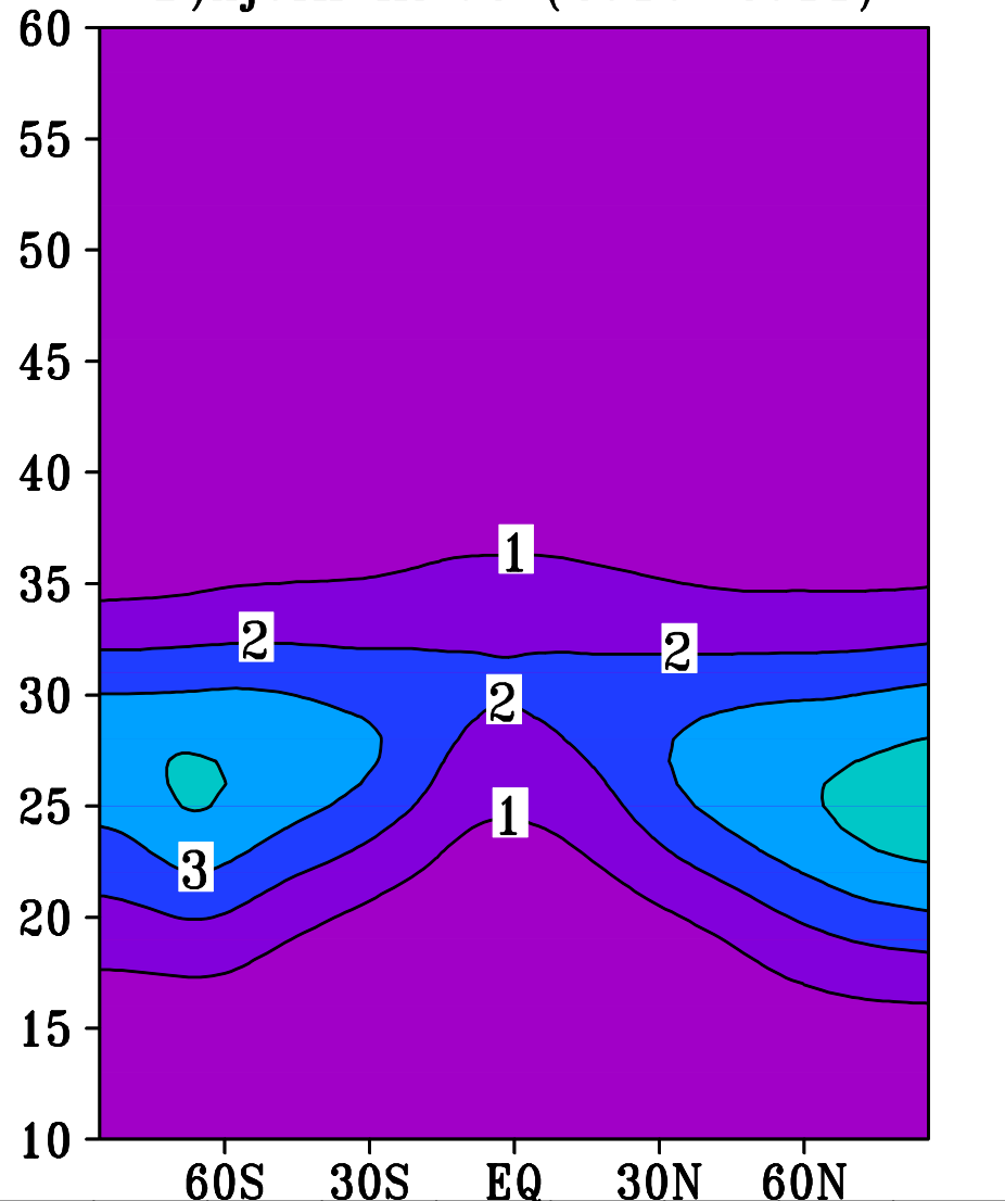
B) xjcin HN03 (2010–2011)
