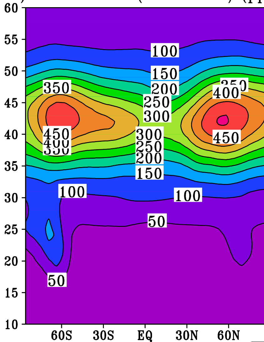
A) SLIMCAT ClO (2010–2011) (ppt)
