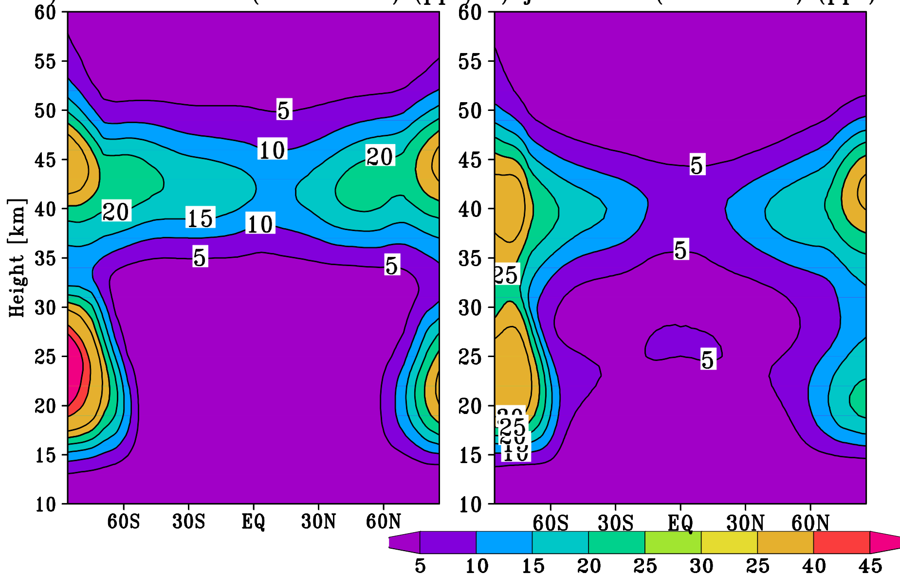
A) SLIMCAT OCL0 (2010–2011) (ppt) B)xjcin OCL0 (2010–2011) (ppt)
