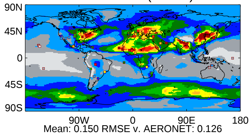
akwxs Total AOD (440nm) JJA
