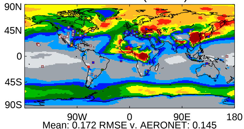
akwxs Total AOD (440nm) DJF
