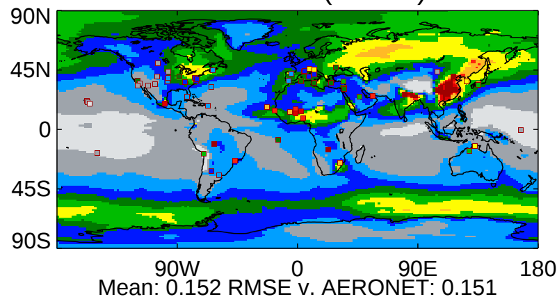
akwxs Total AOD (440nm) SON
