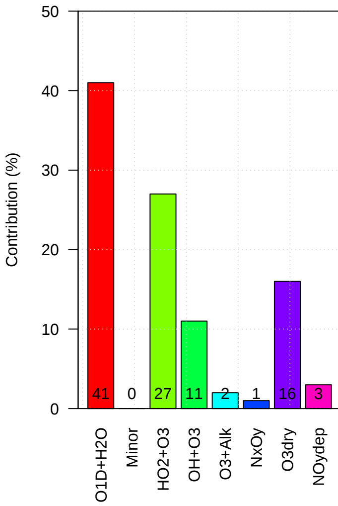
i985a Loss of Tropospheric Ox
