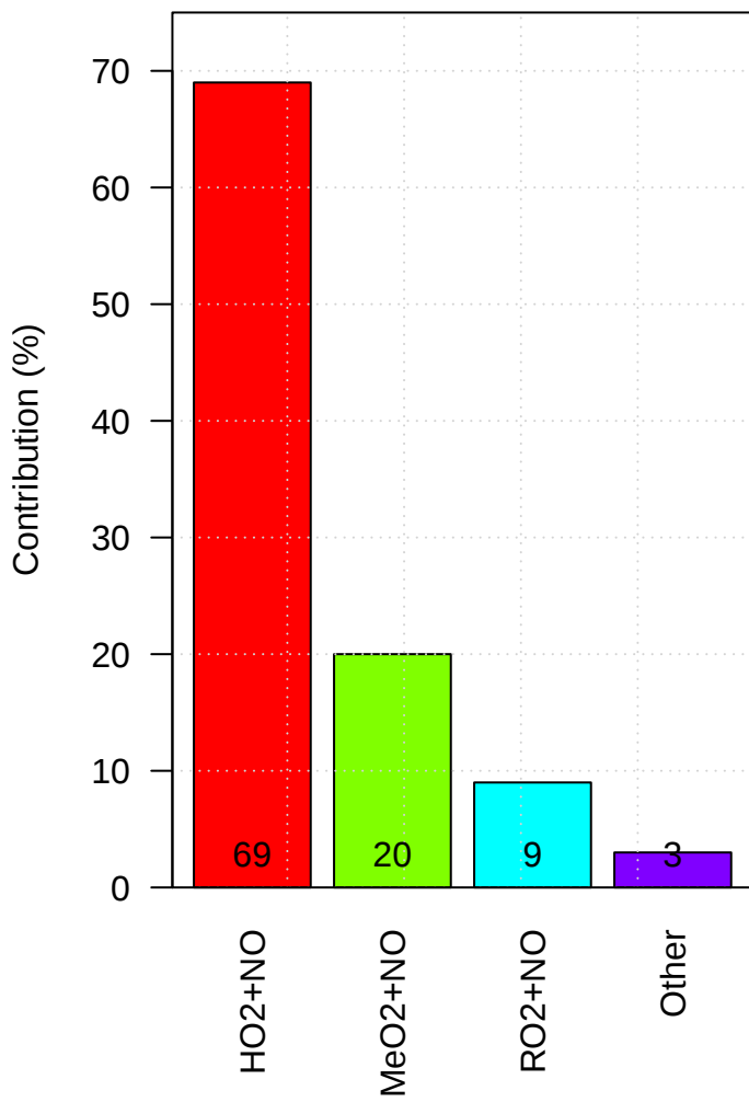
i985a Production of Tropospheric Ox
