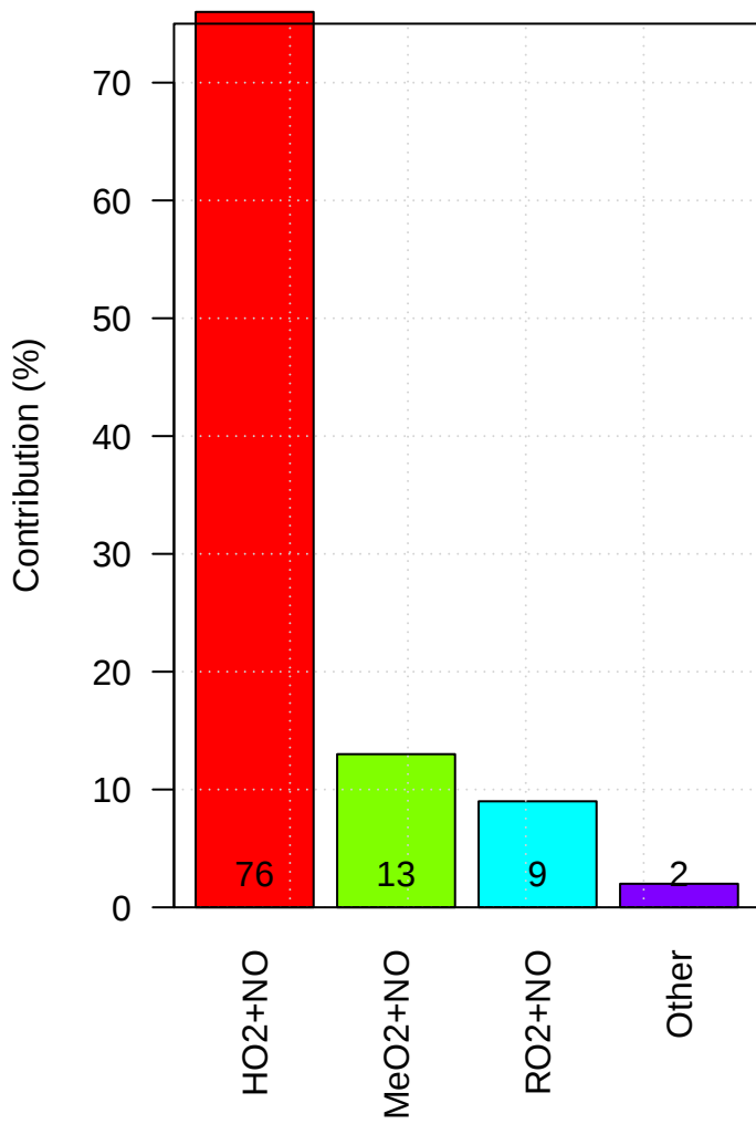
ae771 Production of Tropospheric Ox
