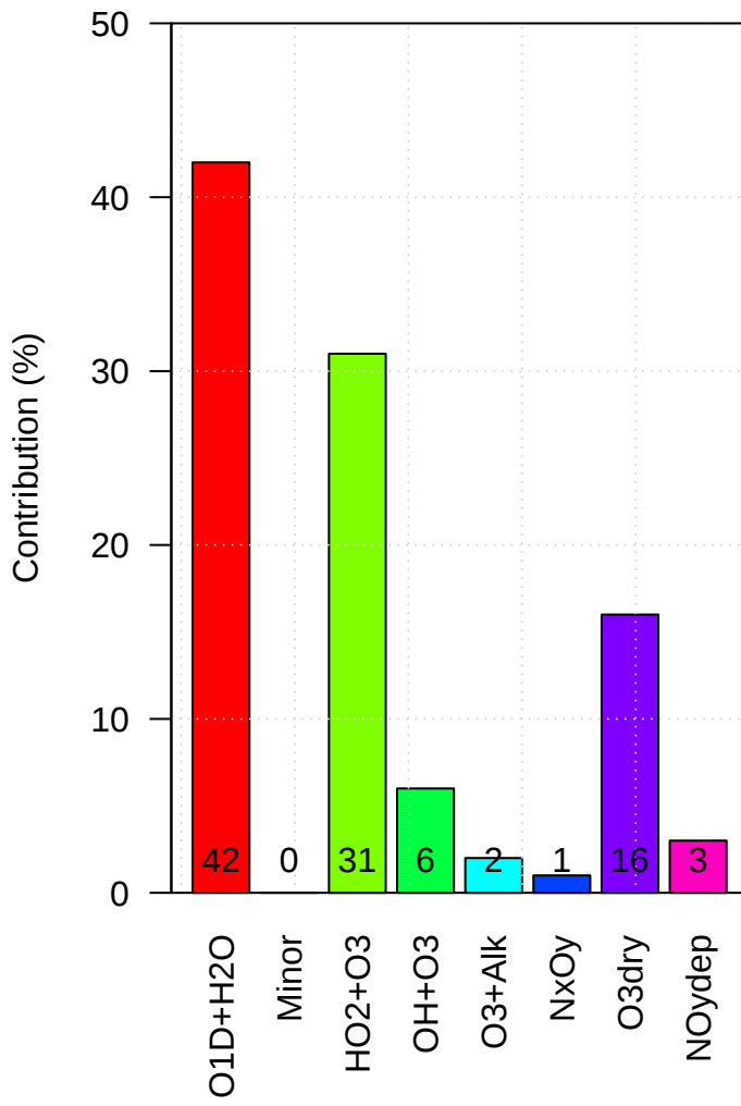
ae771 Loss of Tropospheric Ox
