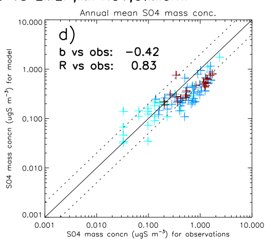
HadGEM3UKCA_BR633_2005 Vs EMEP, IMPROV, U. Miami
