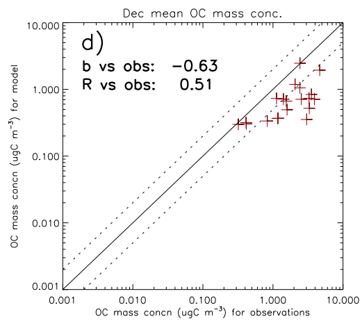
HadGEM3UKCA_BR633_2005 Vs IMPROVE 2000
