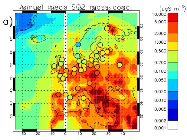
HadGEM3UKCA_BR633_2005 Vs EMEP,CASINET
