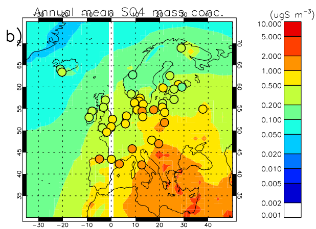
HadGEM3UKCA_BR633_2005 Vs EMEP, IMPROV, U. Miami
