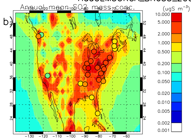
HadGEM3UKCA_BR633_2005 Vs EMEP,CASINET
